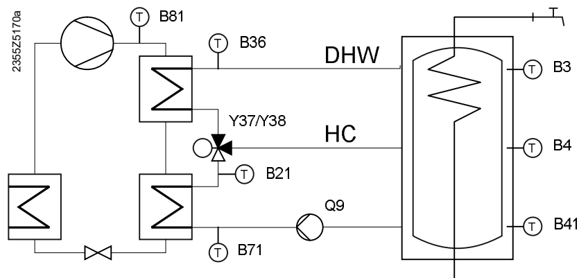
Plant diagram 1: Mixing valve
