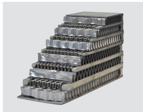
Example of different turbulators
