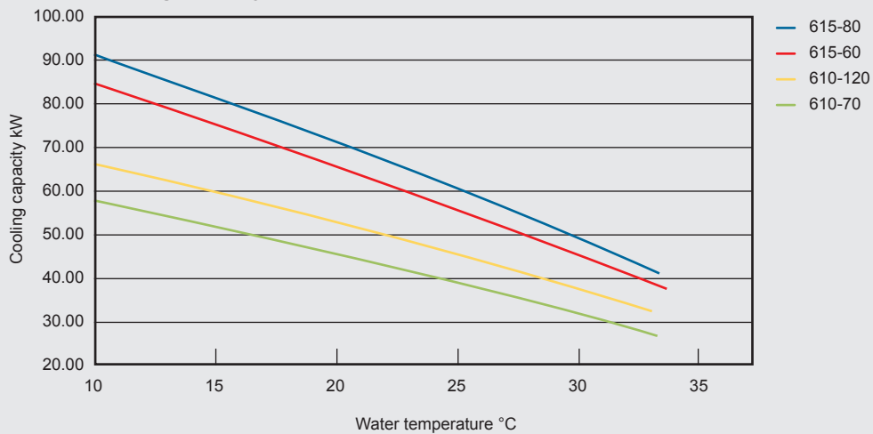
Cooling capacity at 185 l/min
