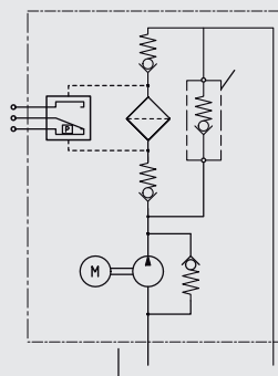
UF (without heat exchanger)
