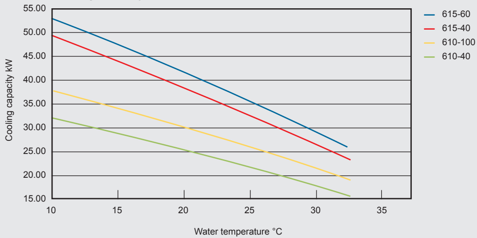
Cooling capacity at 105 l/min
