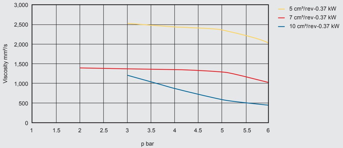
Motor: 0.37 kW
