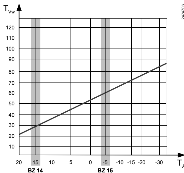
Heating curve diagram showing the basic settings
